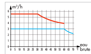
Station BWT ECOBIO 3
